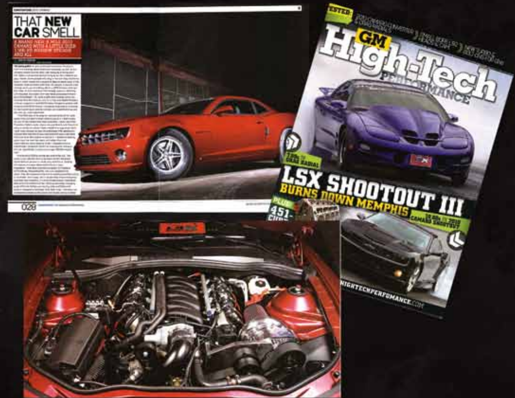
GM High-Tech Performance, March 2010 issue: Starting with a brand new 2010 Camaro SS, David Caine went with a ProCharger Cog Race kit and an intercooled ProCharger F-1C supercharger on a built LS engine to produce 1,048 HP!
